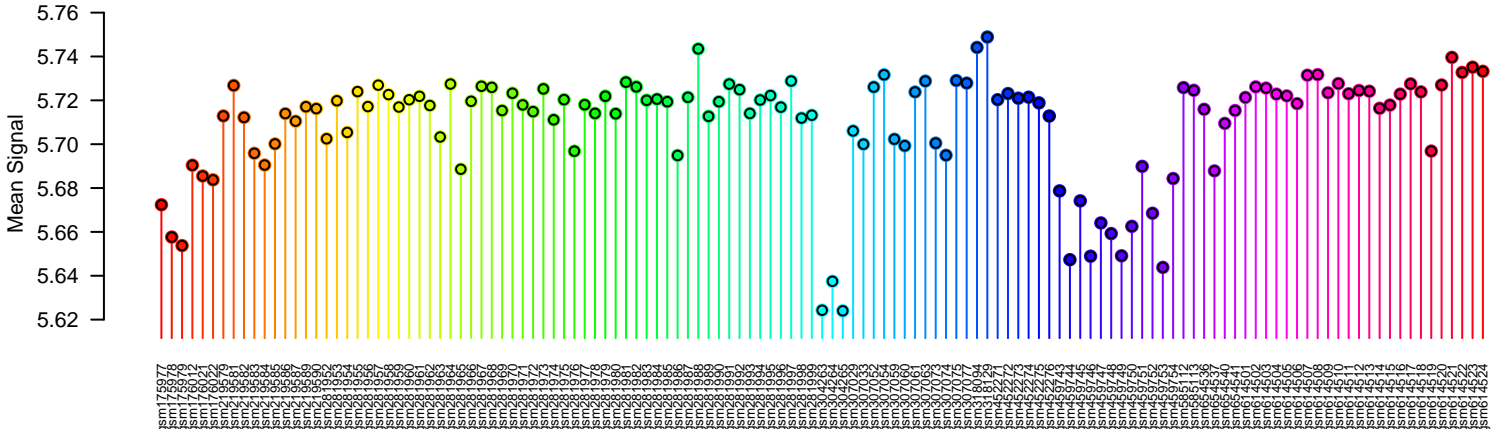
All probsets Mean
