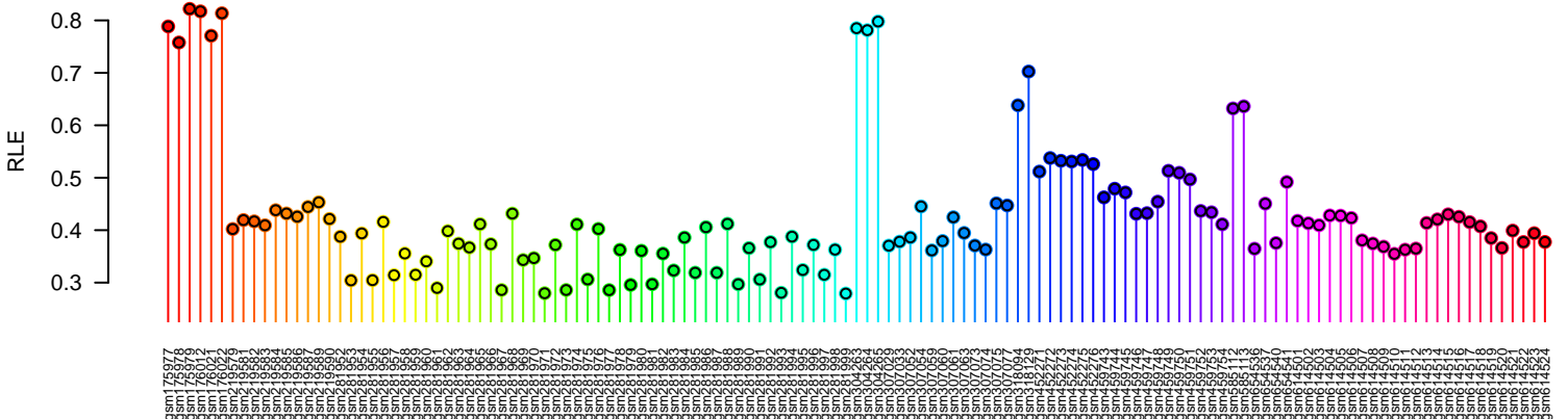
All probsets RLE
